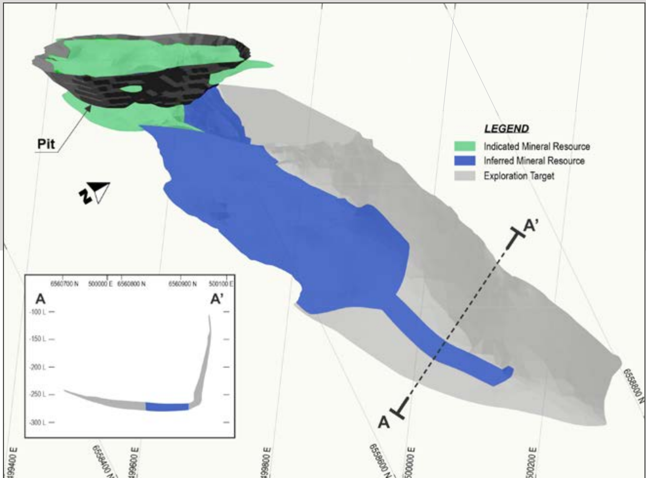
Tritton Project Constellation Deposit (oblique view looking northwest)
