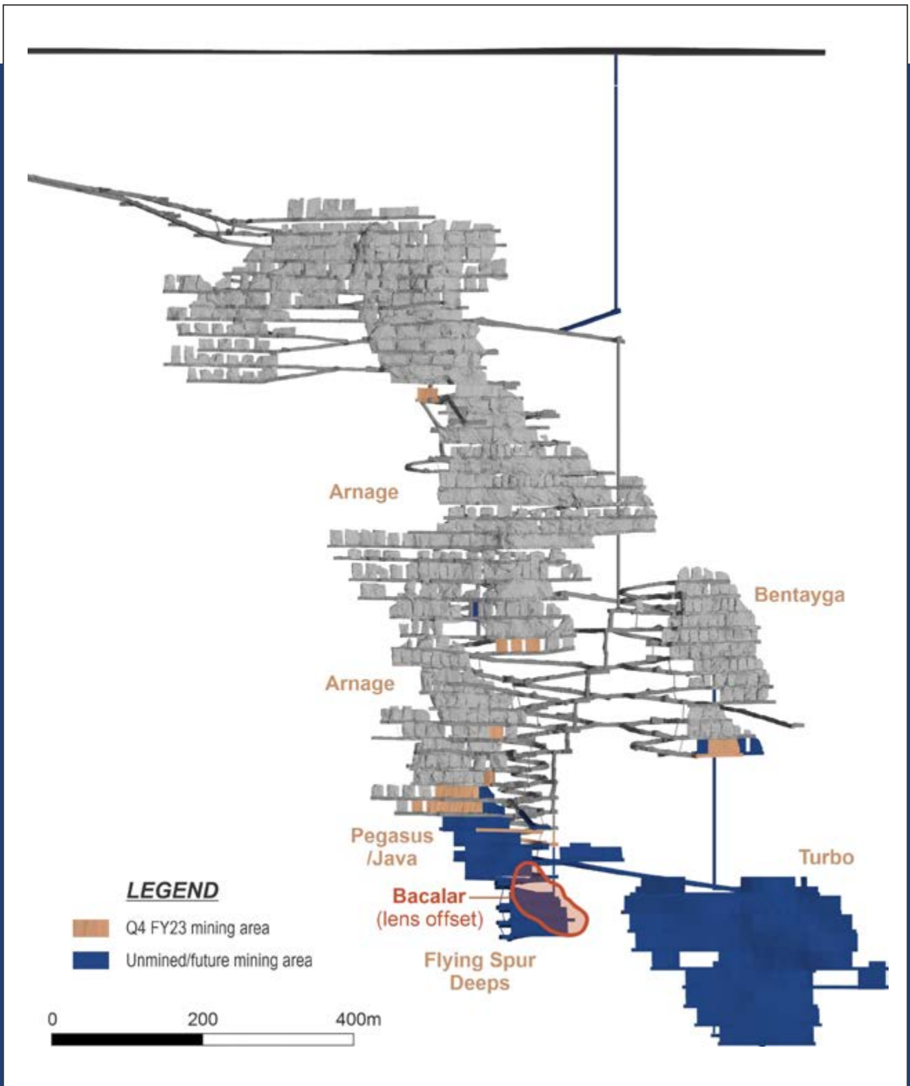
Bentley mine design
