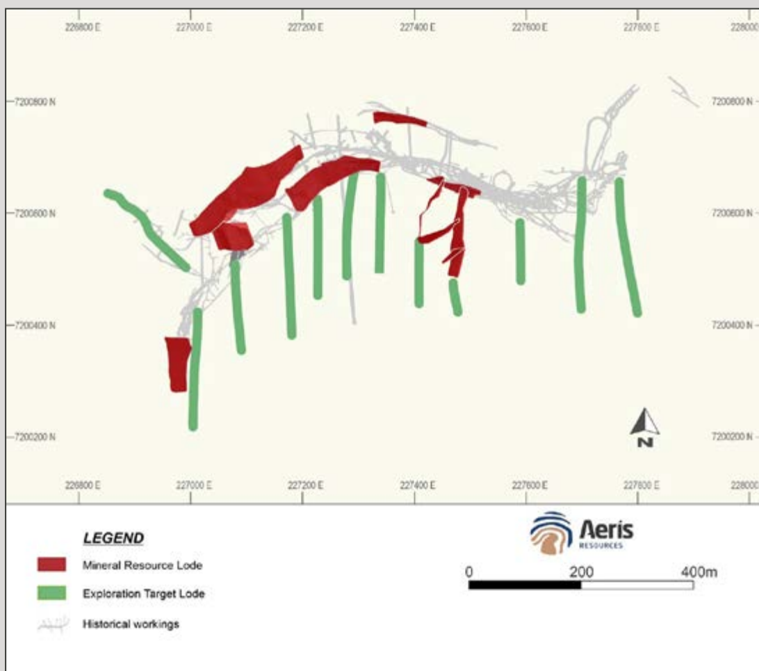
Golden Plateau (Mineral Resource and Exploration Target)
